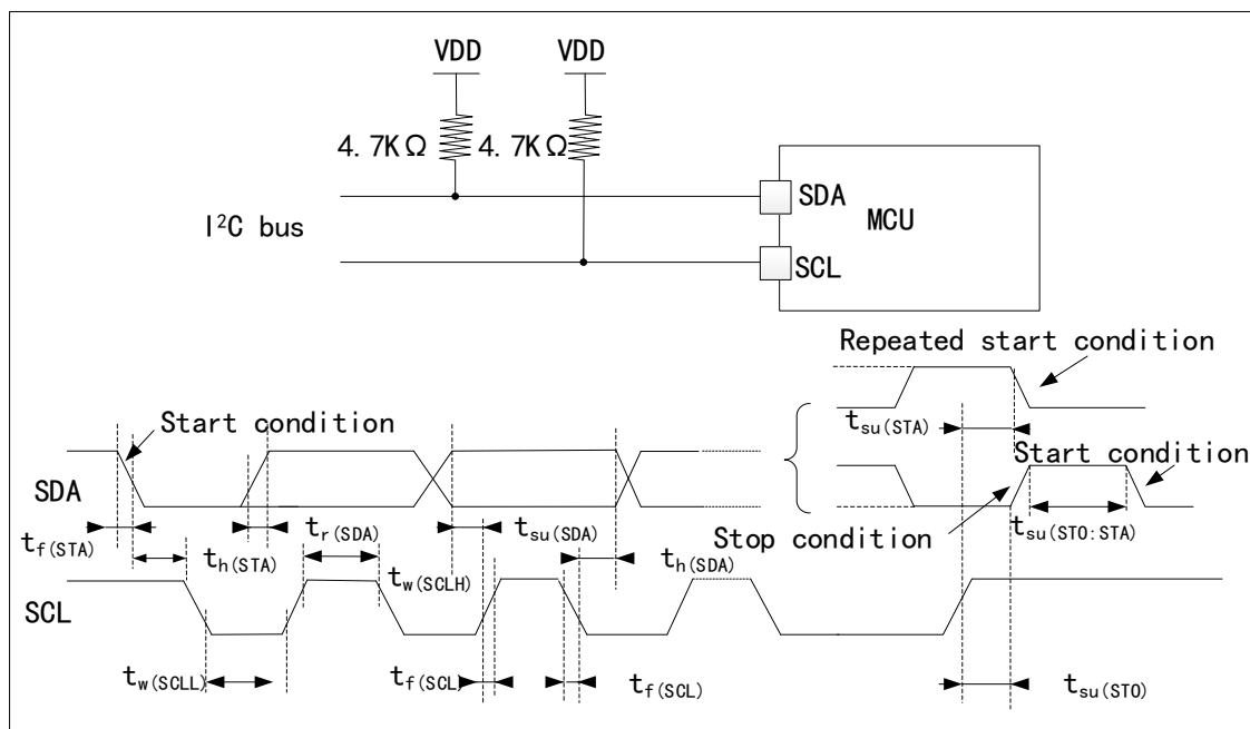
Figure 16 Bus AC Waveform and Measurement Circuit
