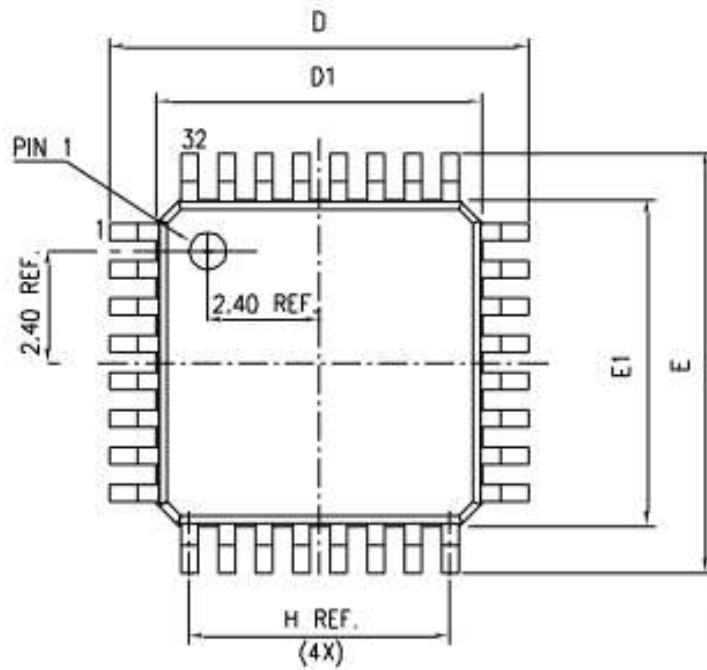
Figure 29 LQFP32 Package Diagram
