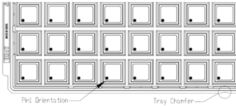
Figure 41 Tray Packaging Diagram
